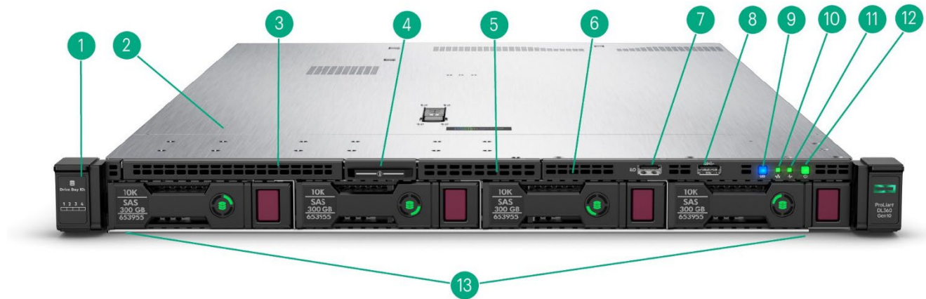
4 LFF Front View – Standard 4 LFF shown
