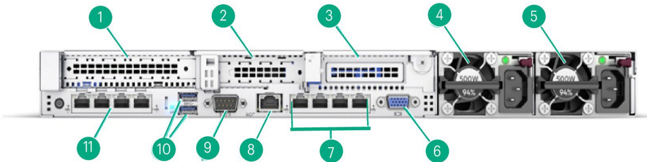
Rear View – Standard for all DL360 Gen10
